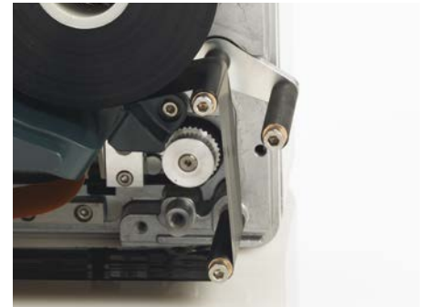
Dancer Arms reduce ribbon tension eliminating ribbon breaks.
